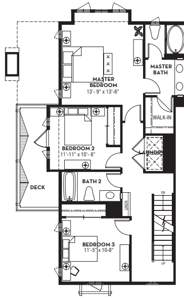
SECOND FLOOR PLAN UNIT OCCURS AT BUILDING 700A
