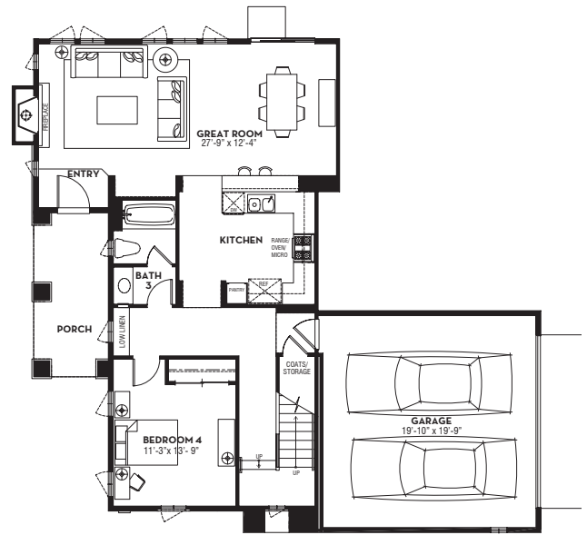
FIRST FLOOR PLAN UNIT OCCURS AT BUILDING 700A
