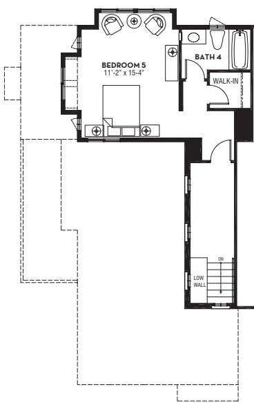
THIRD FLOOR PLAN UNIT OCCURS AT BUILDING 700A
